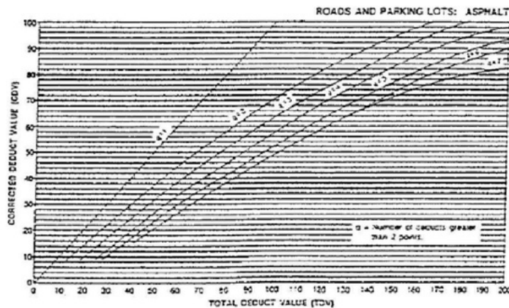
FIGURE 2. The relationship between TDV and CDV [37]
