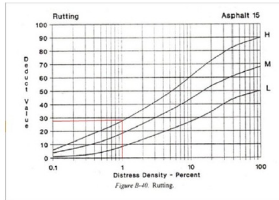
FIGURE 3. The relationship curve between distress density and deduct value for rutting.
