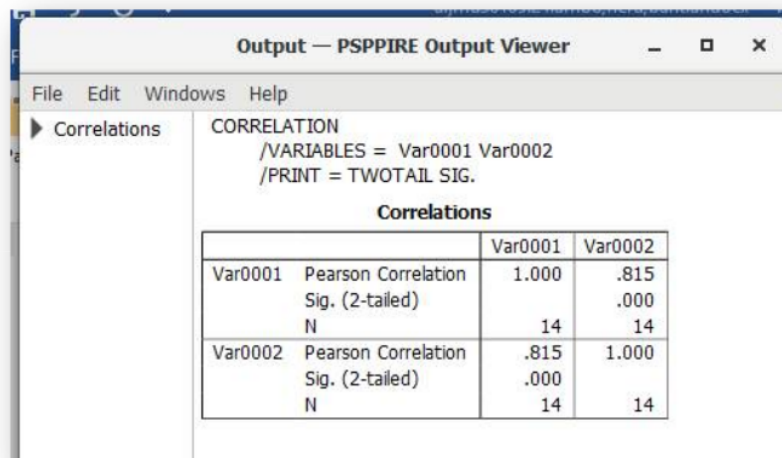
Figure 4. Output of Pearson correlation test using PSPP program (strong correlation)
